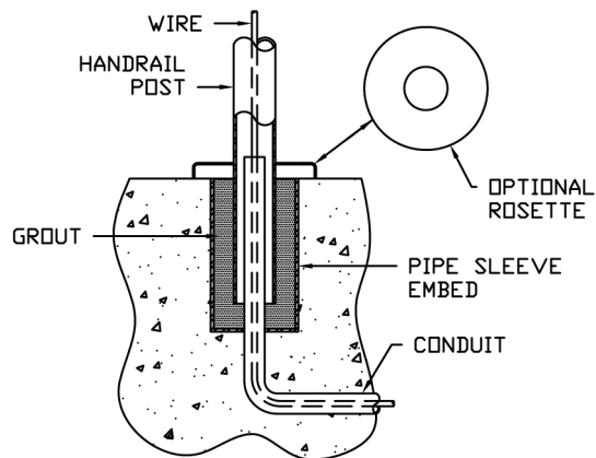
STANDARD POST MOUNTING @ WIRE FEED
