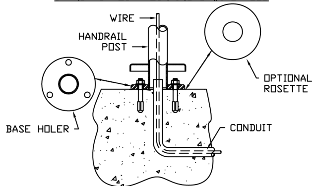
STANDARD POST MOUNTING @ WIRE FEED
