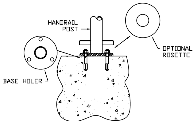
OPTIONAL POST MOUNTING WITH NO WIRE FEED
