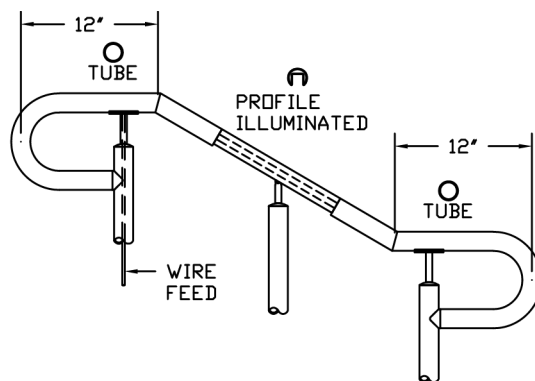
FREESTANDING RAIL WITH TOP AND BOTTOM 180° EXTENSIONS
