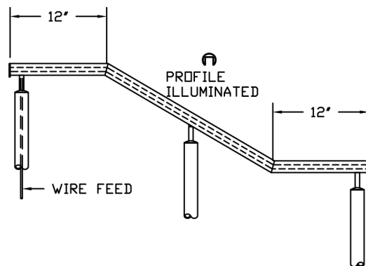
FREESTANDING RAIL WITH TOP AND BOTTOM PROFILE EXTENSIONS
