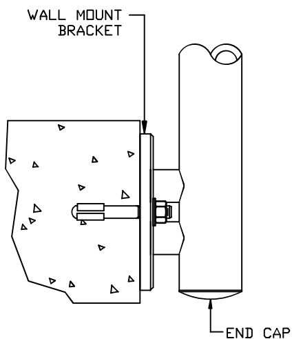
SIDE MOUNT OPTION
