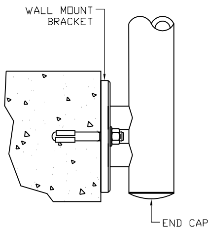
SIDE MOUNT OPTION
