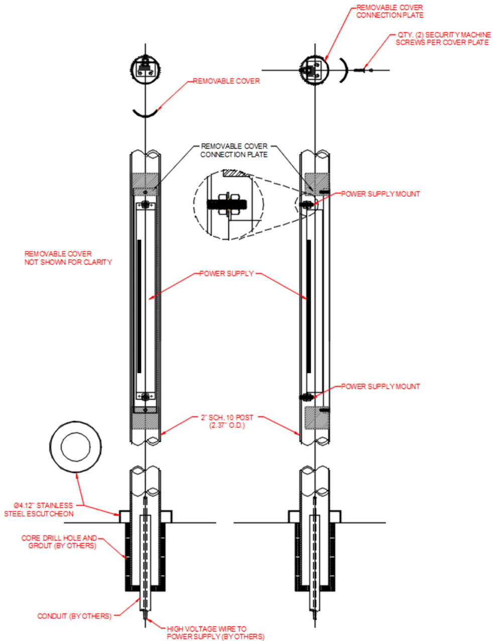
TYPICAL POST WITH INTEGRAL DRIVER DETAIL SCALE: 3" = 1'-0"
